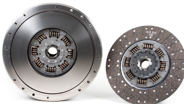
Fig. 2: LuK double disc clutch with same hub profiles
